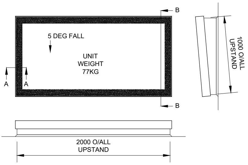
PLAN AND ELEVATIONS SCALE 1:30 (A3)
